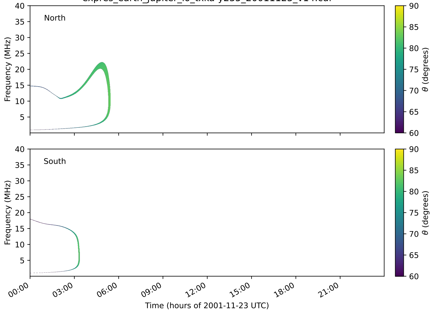
expres_earth_jupiter_io_txka-y235_20011123_v14.cdf
