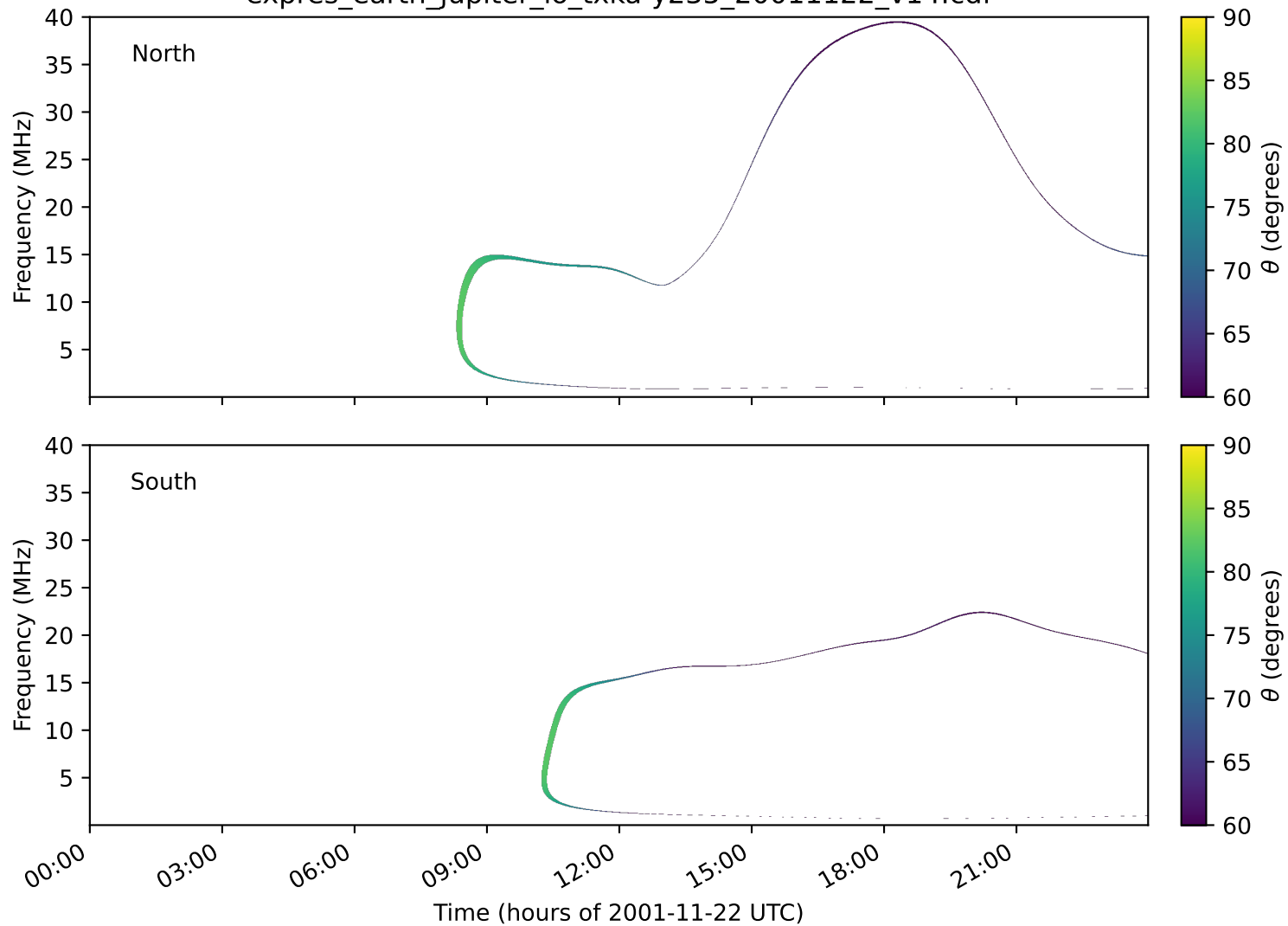
expres_earth_jupiter_io_txka-y235_20011122_v14.cdf
