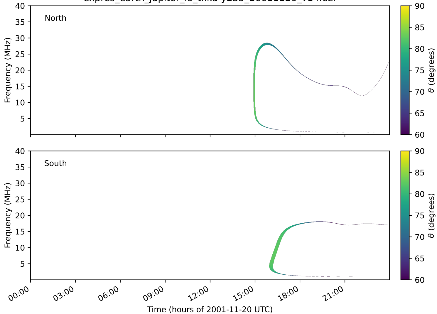
expres_earth_jupiter_io_txka-y235_20011120_v14.cdf
