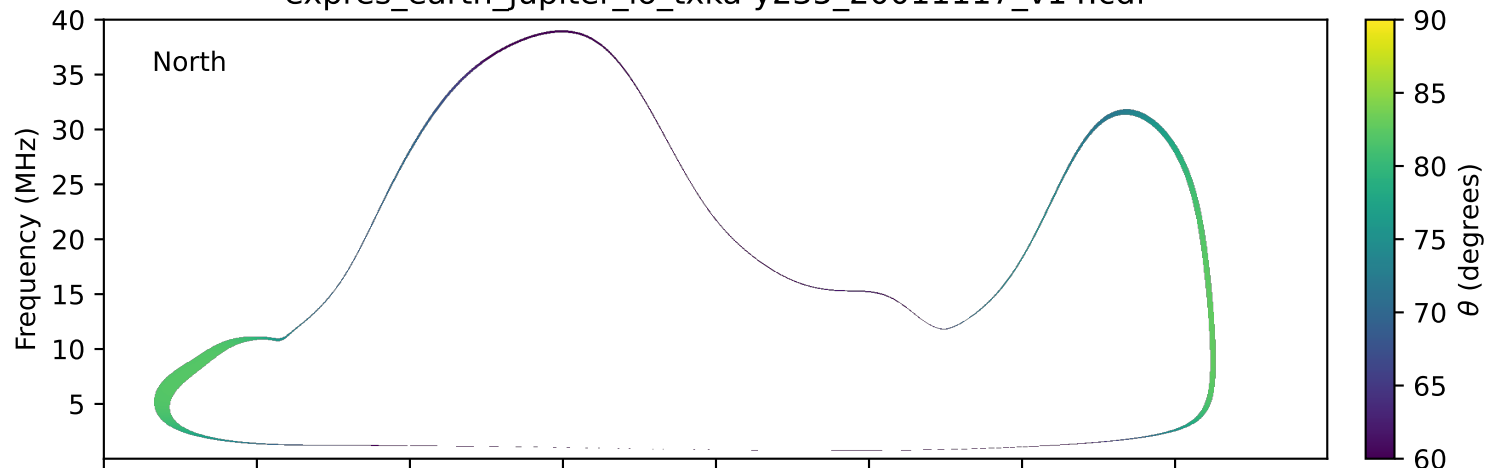
expres_earth_jupiter_io_txka-y235_20011117_v14.cdf
