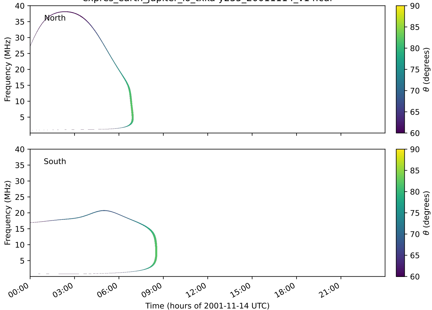
expres_earth_jupiter_io_txka-y235_20011114_v14.cdf
