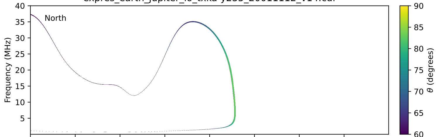
expres_earth_jupiter_io_txka-y235_20011112_v14.cdf
