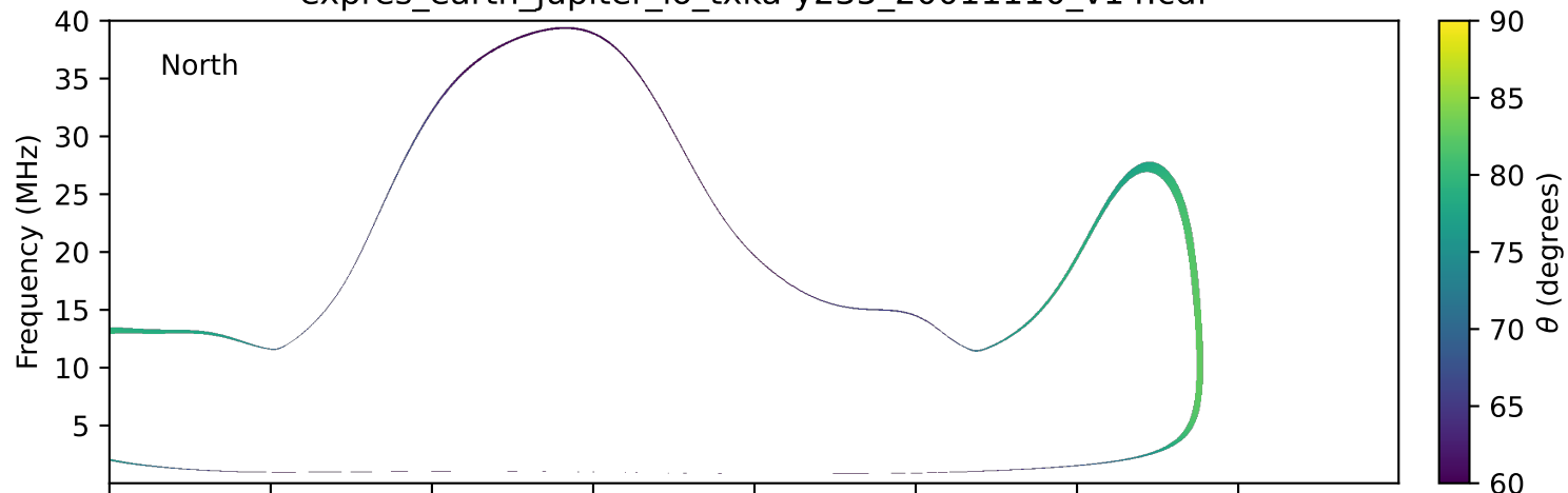
expres_earth_jupiter_io_txka-y235_20011110_v14.cdf
