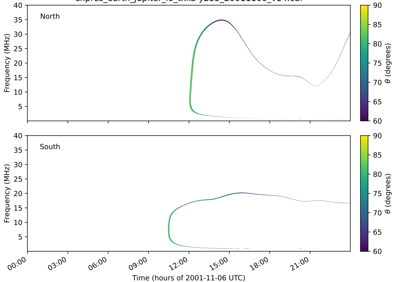
expres_earth_jupiter_io_txka-y235_20011106_v14.cdf
