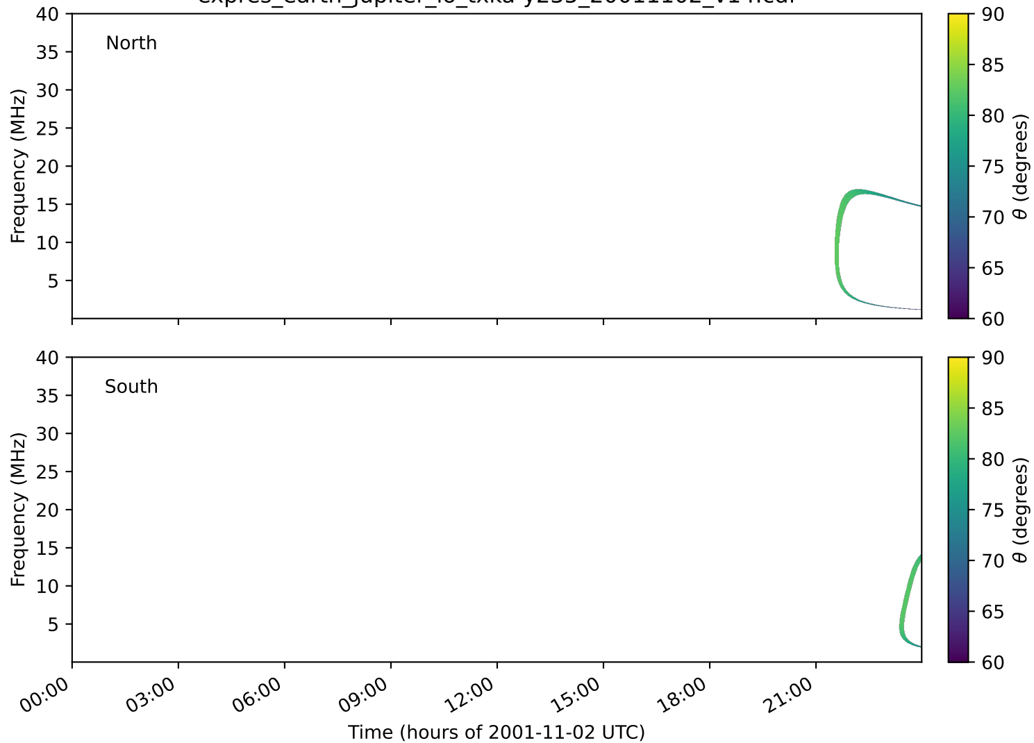
expres_earth_jupiter_io_txka-y235_20011102_v14.cdf
