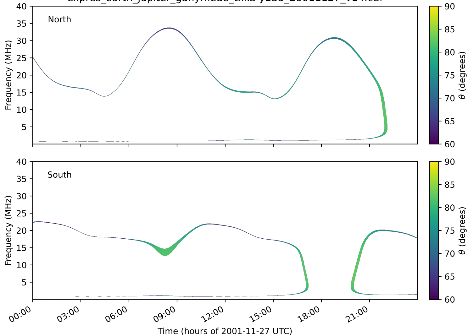
expres_earth_jupiter_ganymede_txka-y235_20011127_v14.cdf
