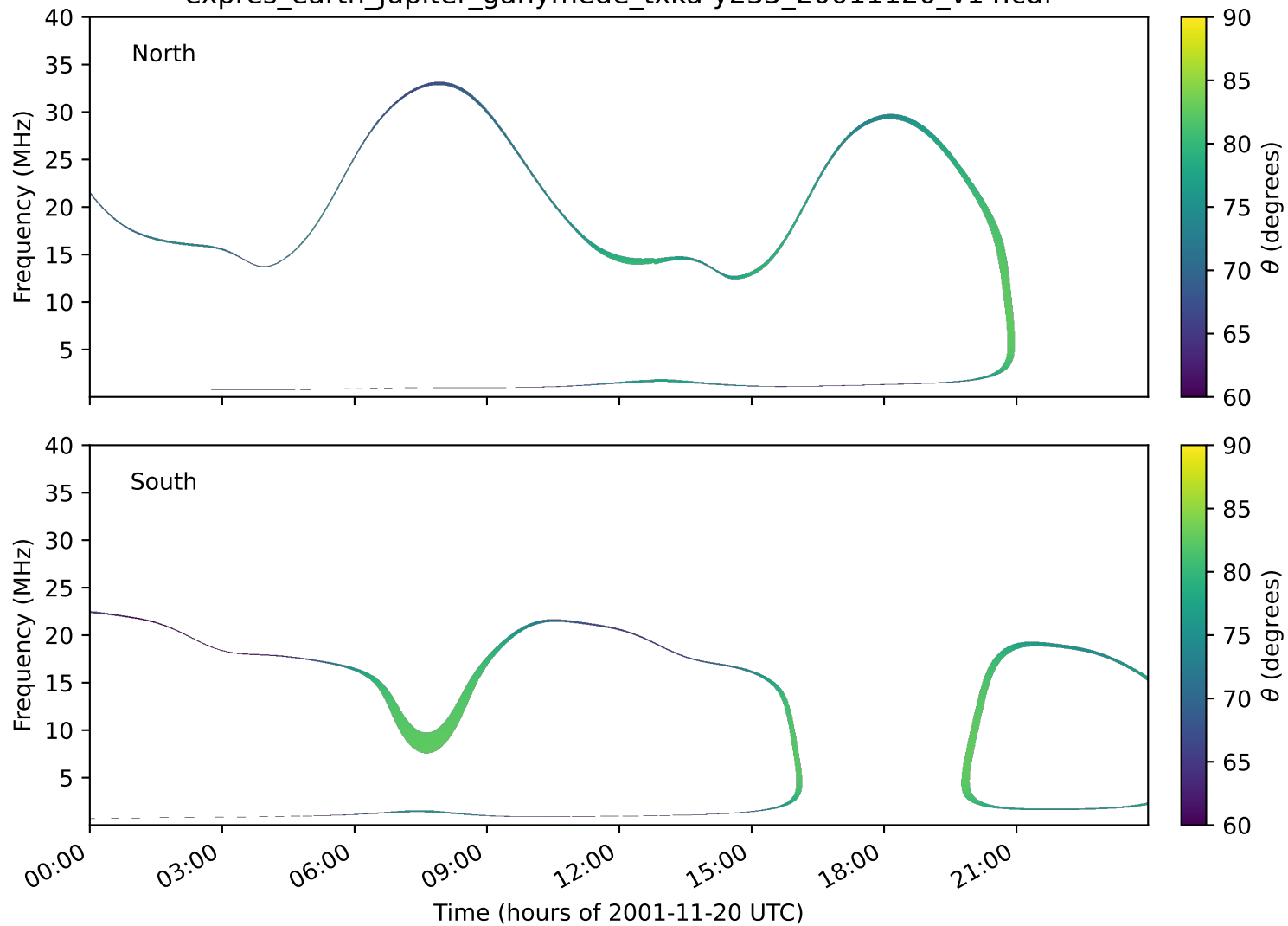
expres_earth_jupiter_ganymede_txka-y235_20011120_v14.cdf
