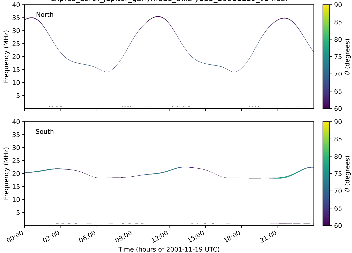
expres_earth_jupiter_ganymede_txka-y235_20011119_v14.cdf
