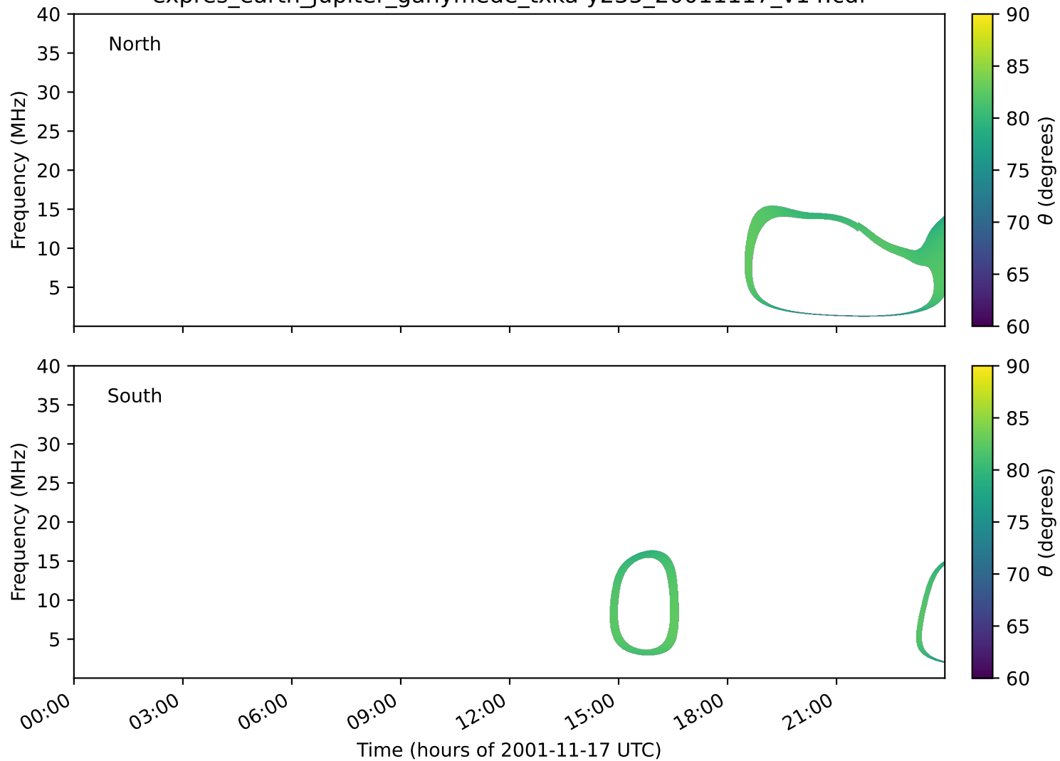
expres_earth_jupiter_ganymede_txka-y235_20011117_v14.cdf
