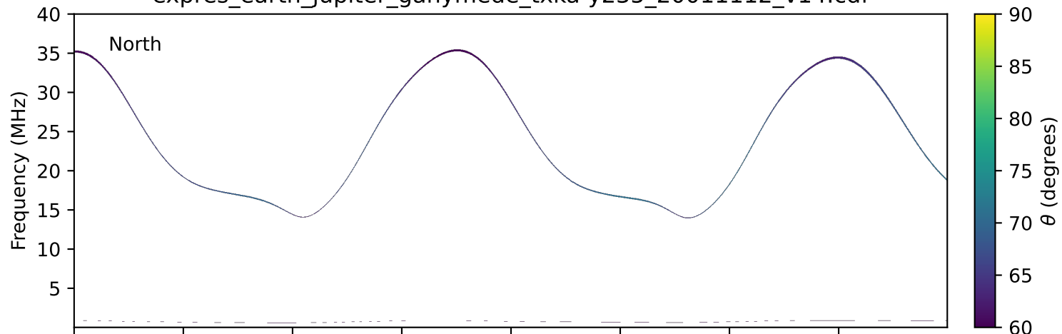
expres_earth_jupiter_ganymede_txka-y235_20011112_v14.cdf
