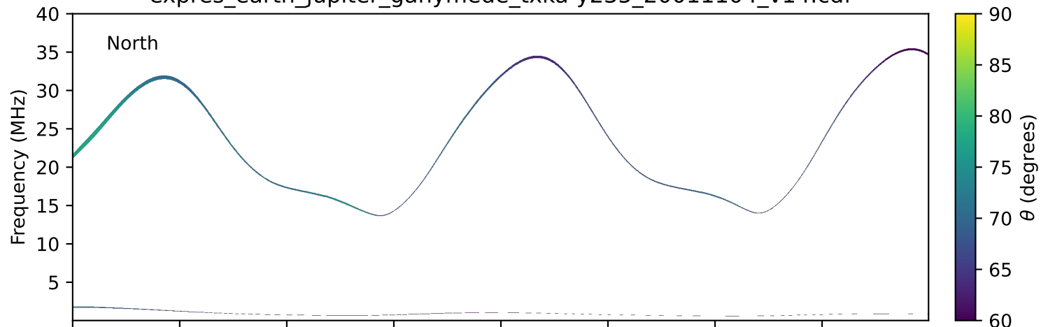
expres_earth_jupiter_ganymede_txka-y235_20011104_v14.cdf
