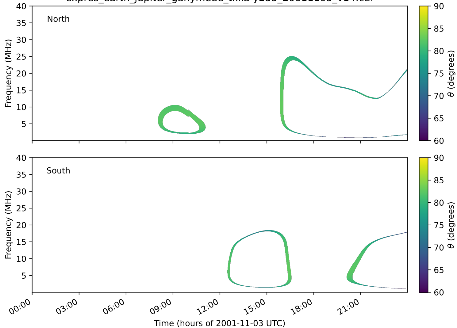
expres_earth_jupiter_ganymede_txka-y235_20011103_v14.cdf
