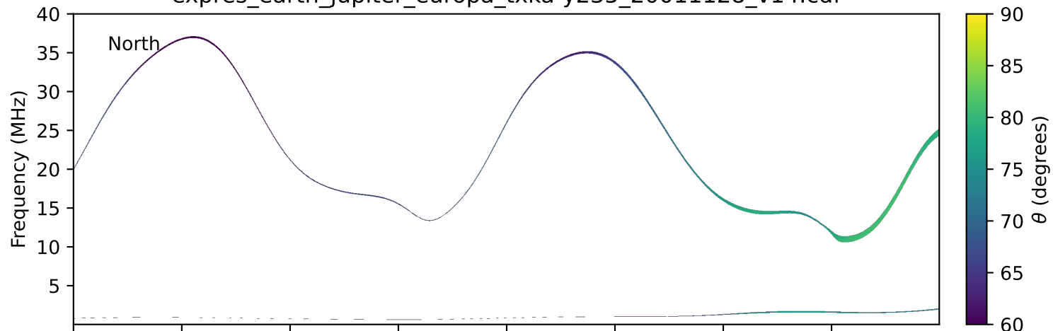
expres_earth_jupiter_europa_txka-y235_20011128_v14.cdf
