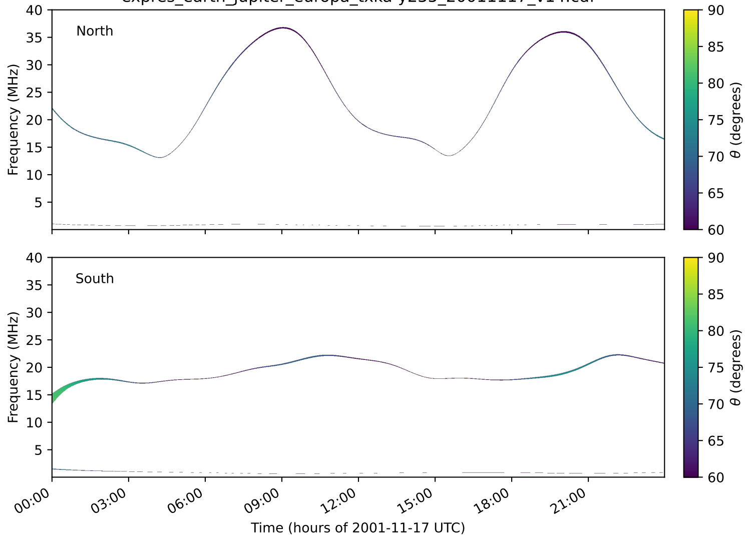
expres_earth_jupiter_europa_txka-y235_20011117_v14.cdf
