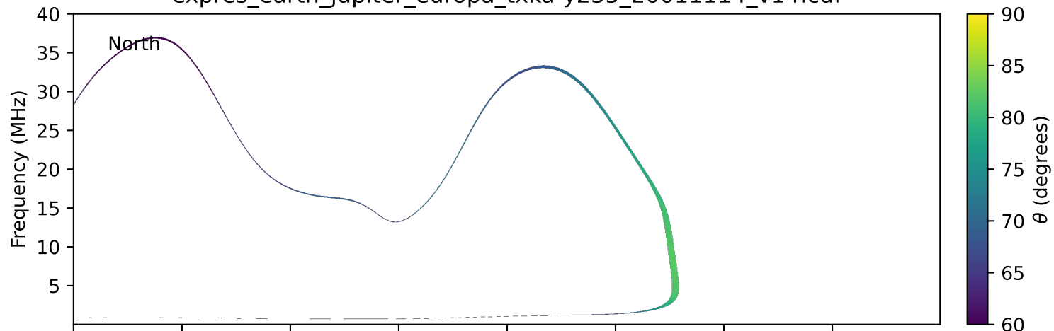
expres_earth_jupiter_europa_txka-y235_20011114_v14.cdf
