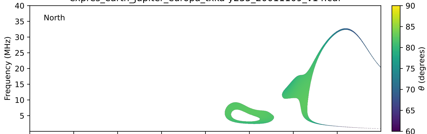
expres_earth_jupiter_europa_txka-y235_20011109_v14.cdf
