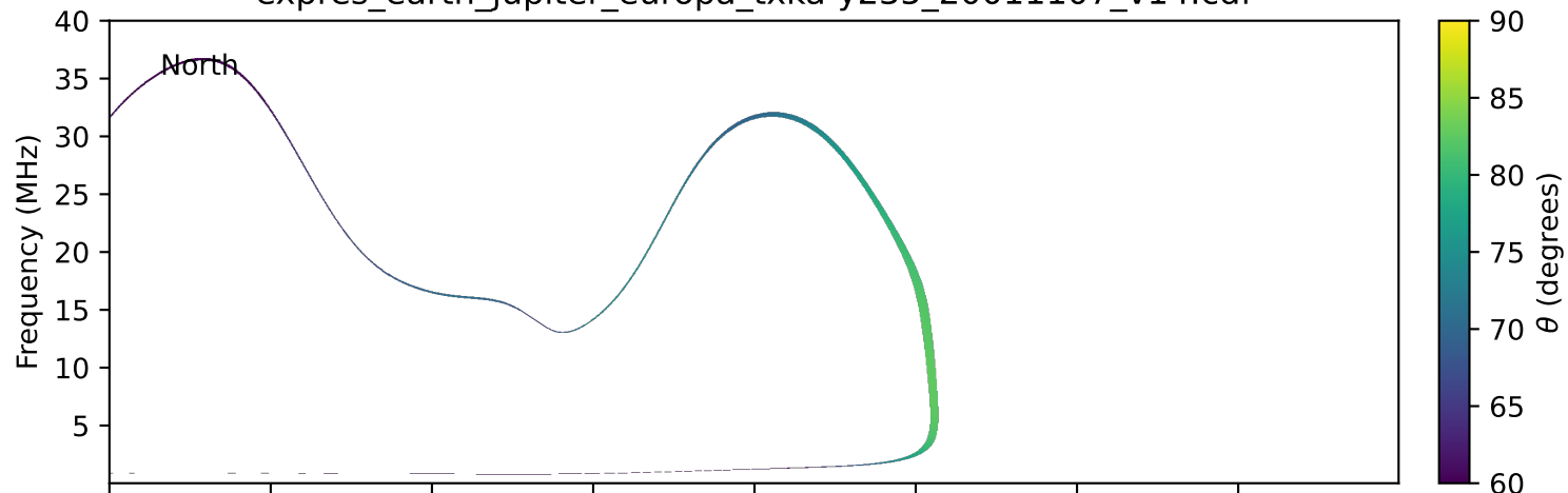
expres_earth_jupiter_europa_txka-y235_20011107_v14.cdf
