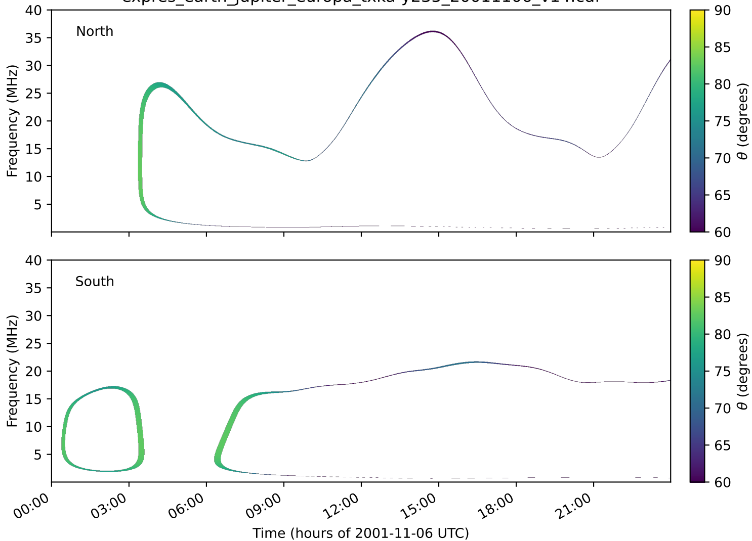
expres_earth_jupiter_europa_txka-y235_20011106_v14.cdf
