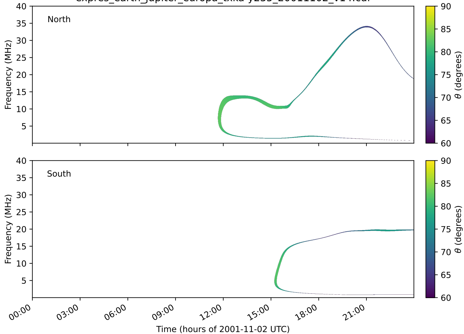
expres_earth_jupiter_europa_txka-y235_20011102_v14.cdf
