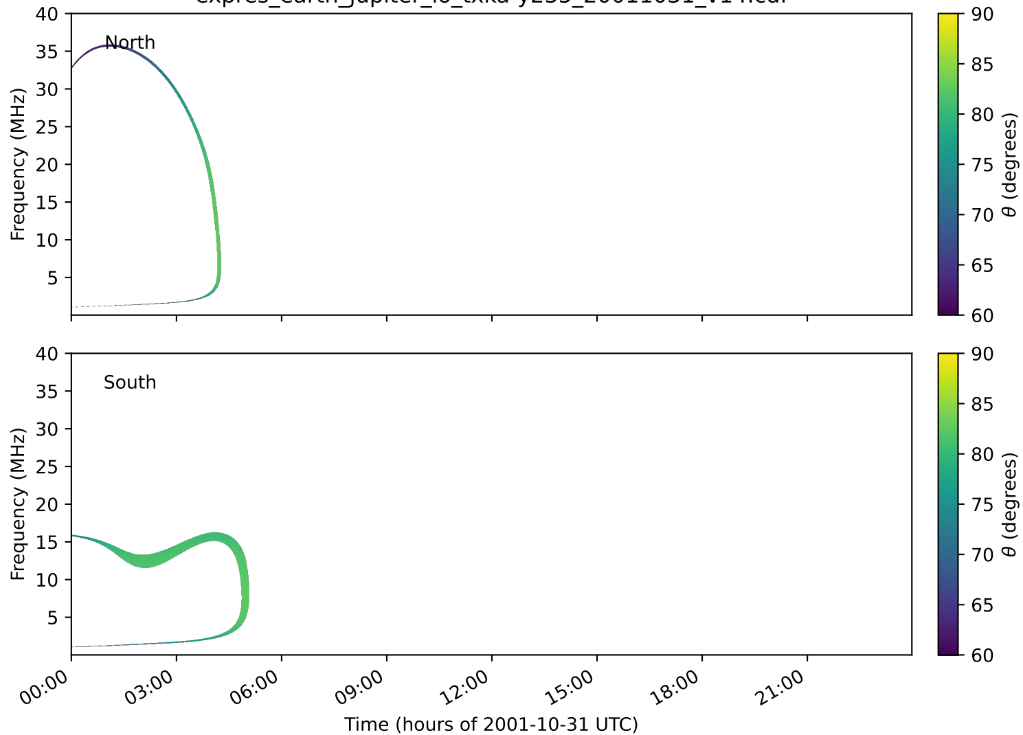
expres_earth_jupiter_io_txka-y235_20011031_v14.cdf
