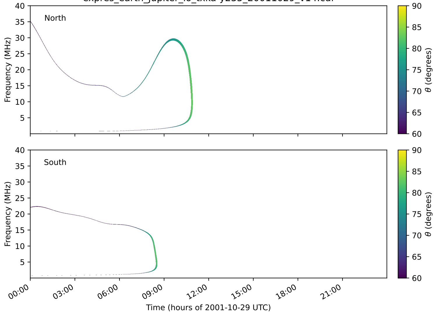
expres_earth_jupiter_io_txka-y235_20011029_v14.cdf
