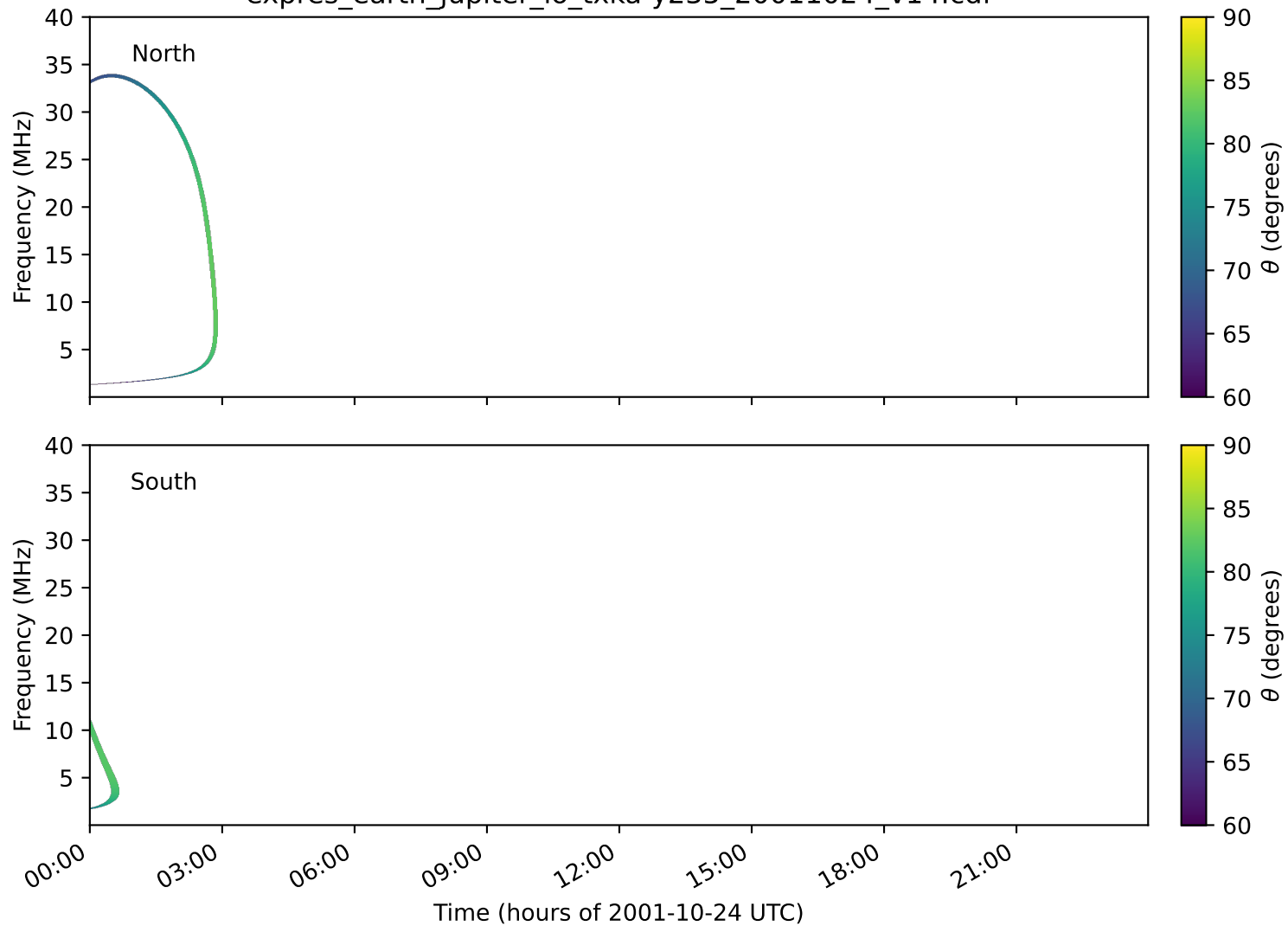
expres_earth_jupiter_io_txka-y235_20011024_v14.cdf
