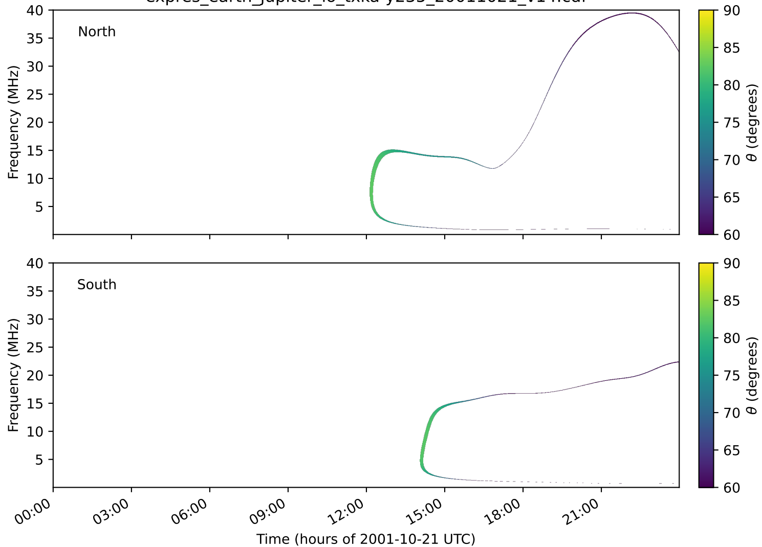
expres_earth_jupiter_io_txka-y235_20011021_v14.cdf
