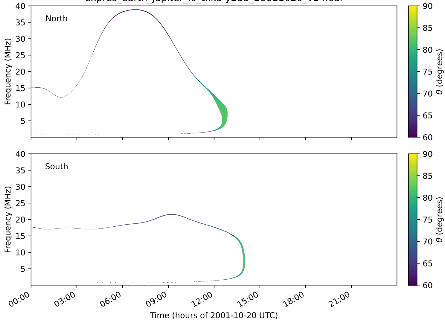
expres_earth_jupiter_io_txka-y235_20011020_v14.cdf
