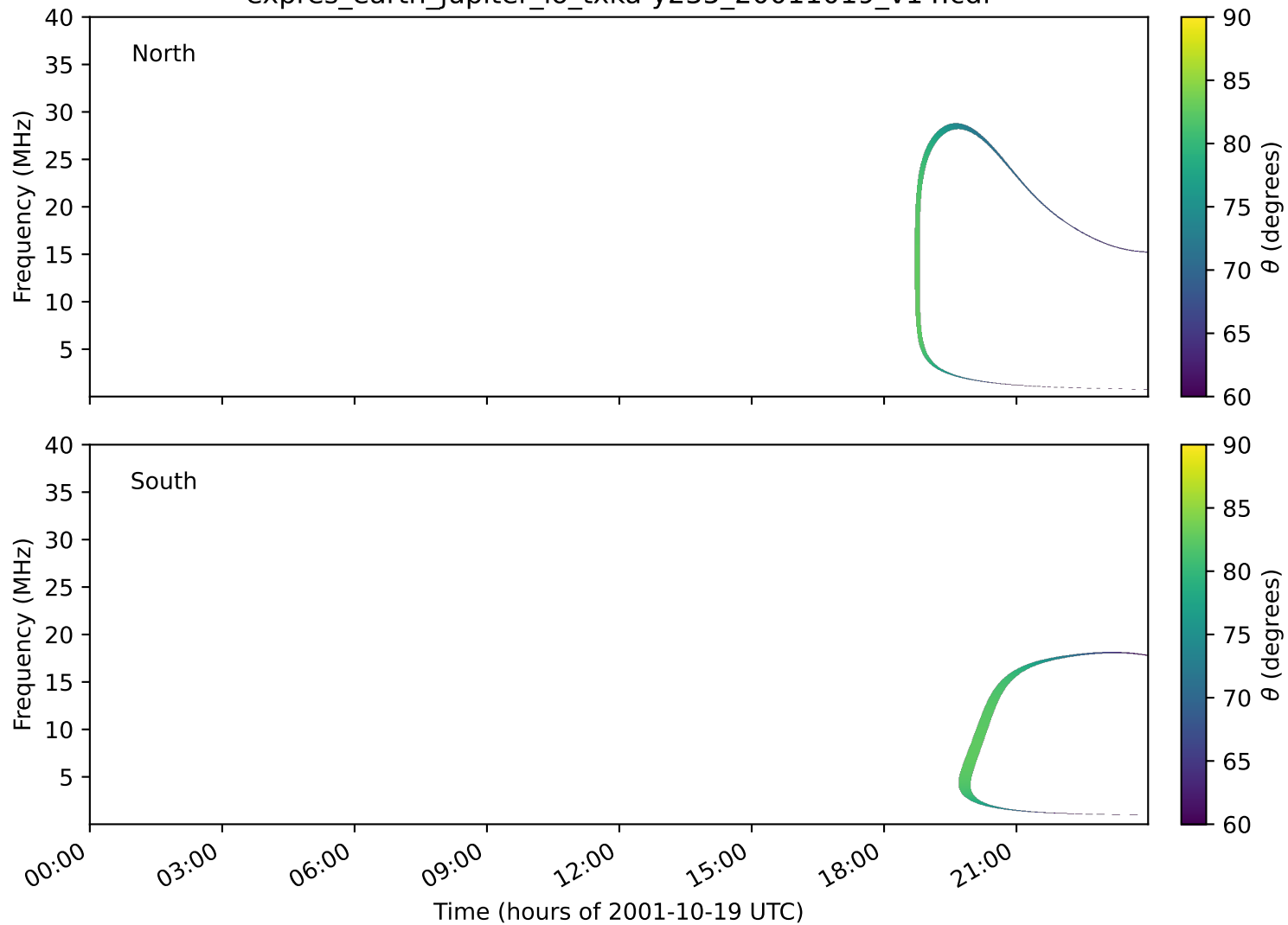
expres_earth_jupiter_io_txka-y235_20011019_v14.cdf
