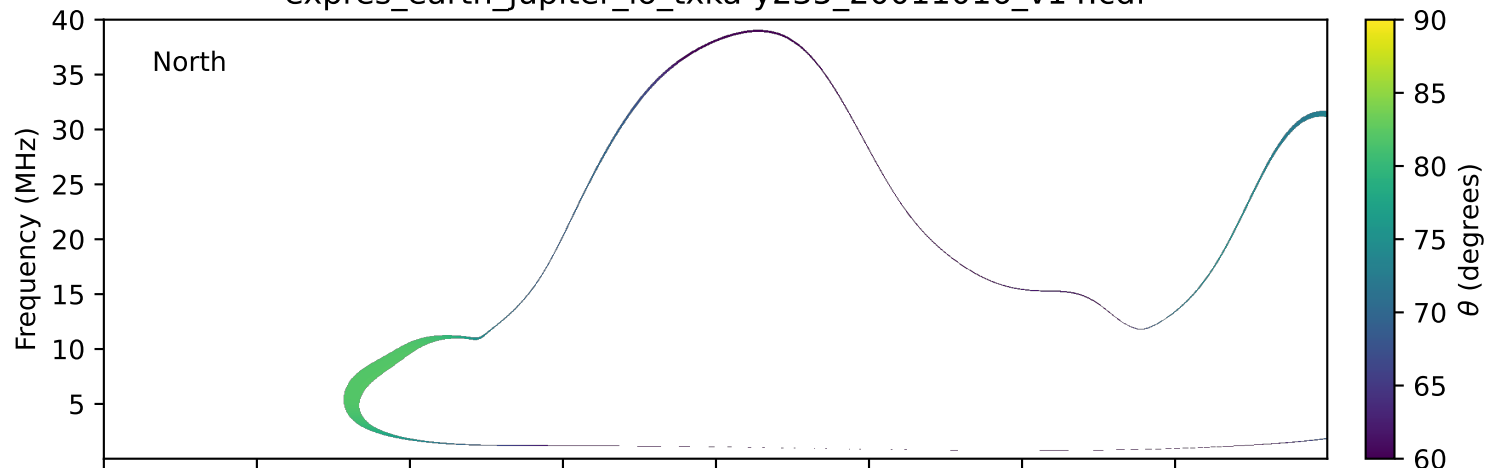
expres_earth_jupiter_io_txka-y235_20011016_v14.cdf
