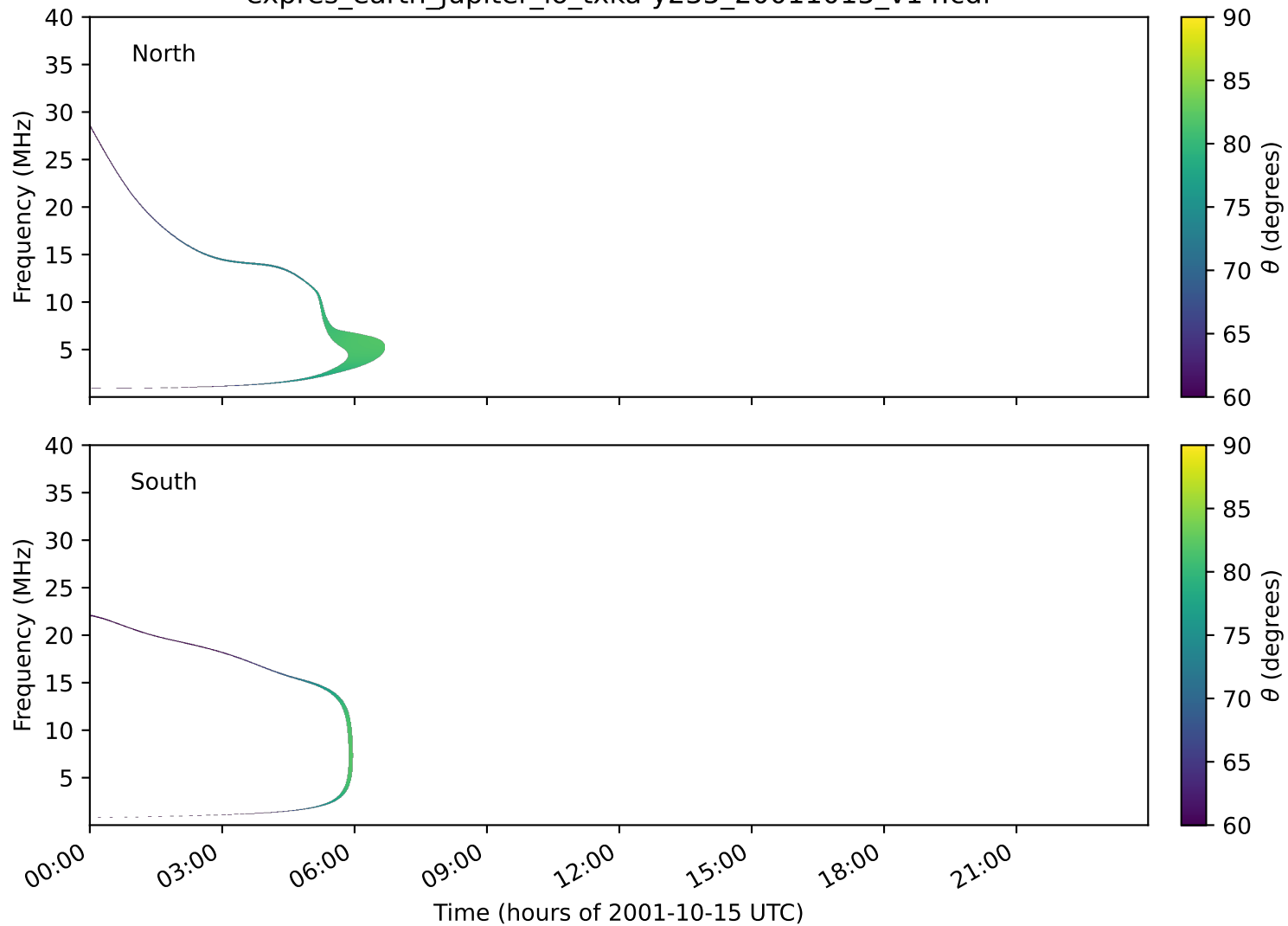
expres_earth_jupiter_io_txka-y235_20011015_v14.cdf
