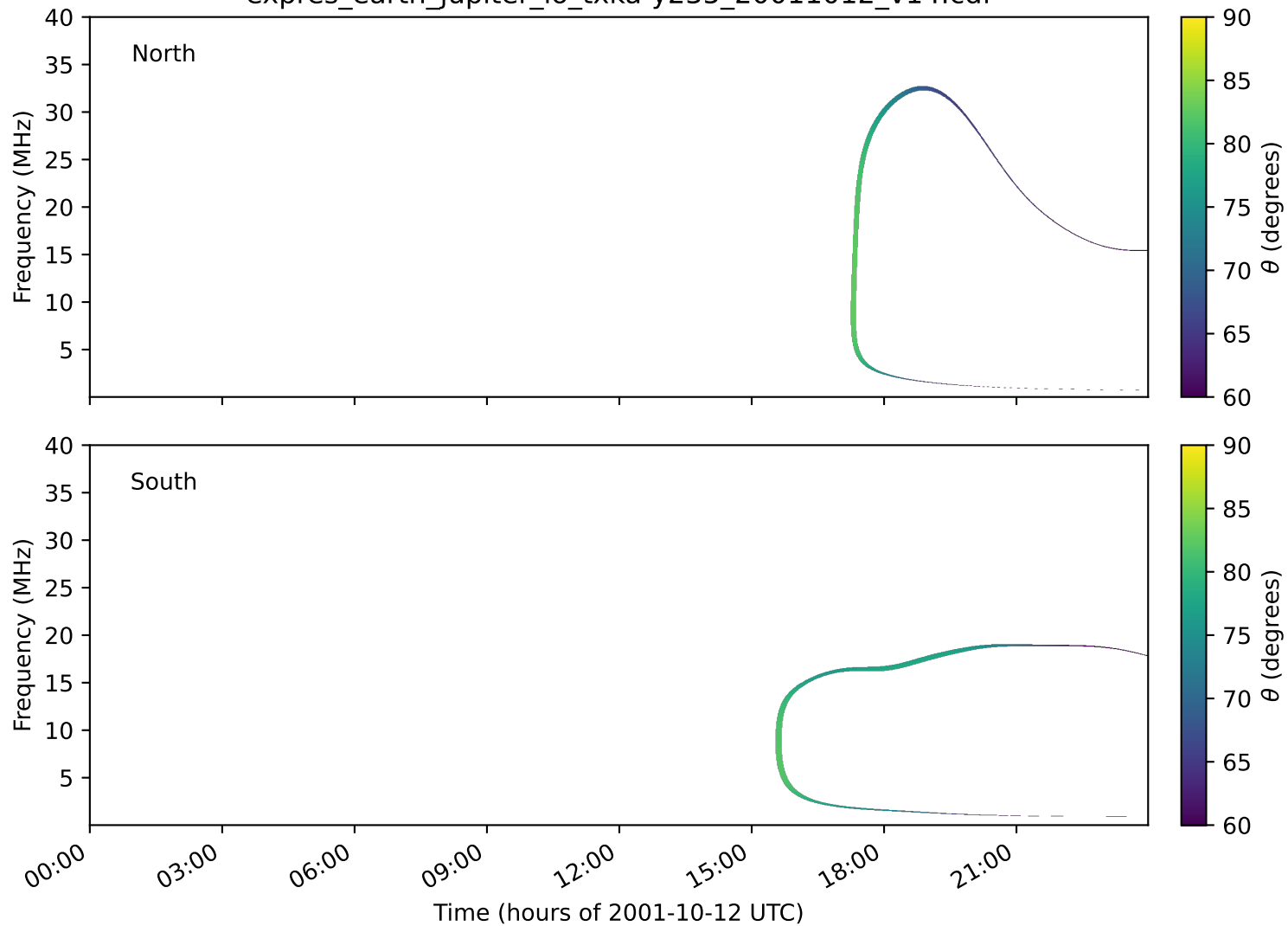
expres_earth_jupiter_io_txka-y235_20011012_v14.cdf
