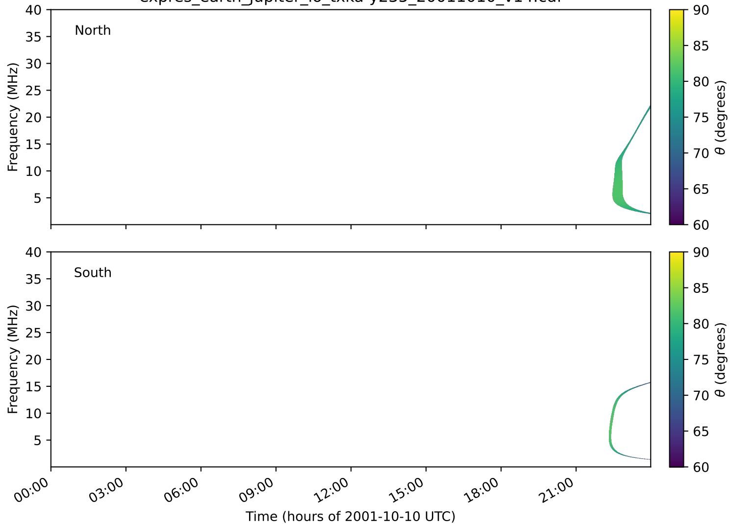
expres_earth_jupiter_io_txka-y235_20011010_v14.cdf
