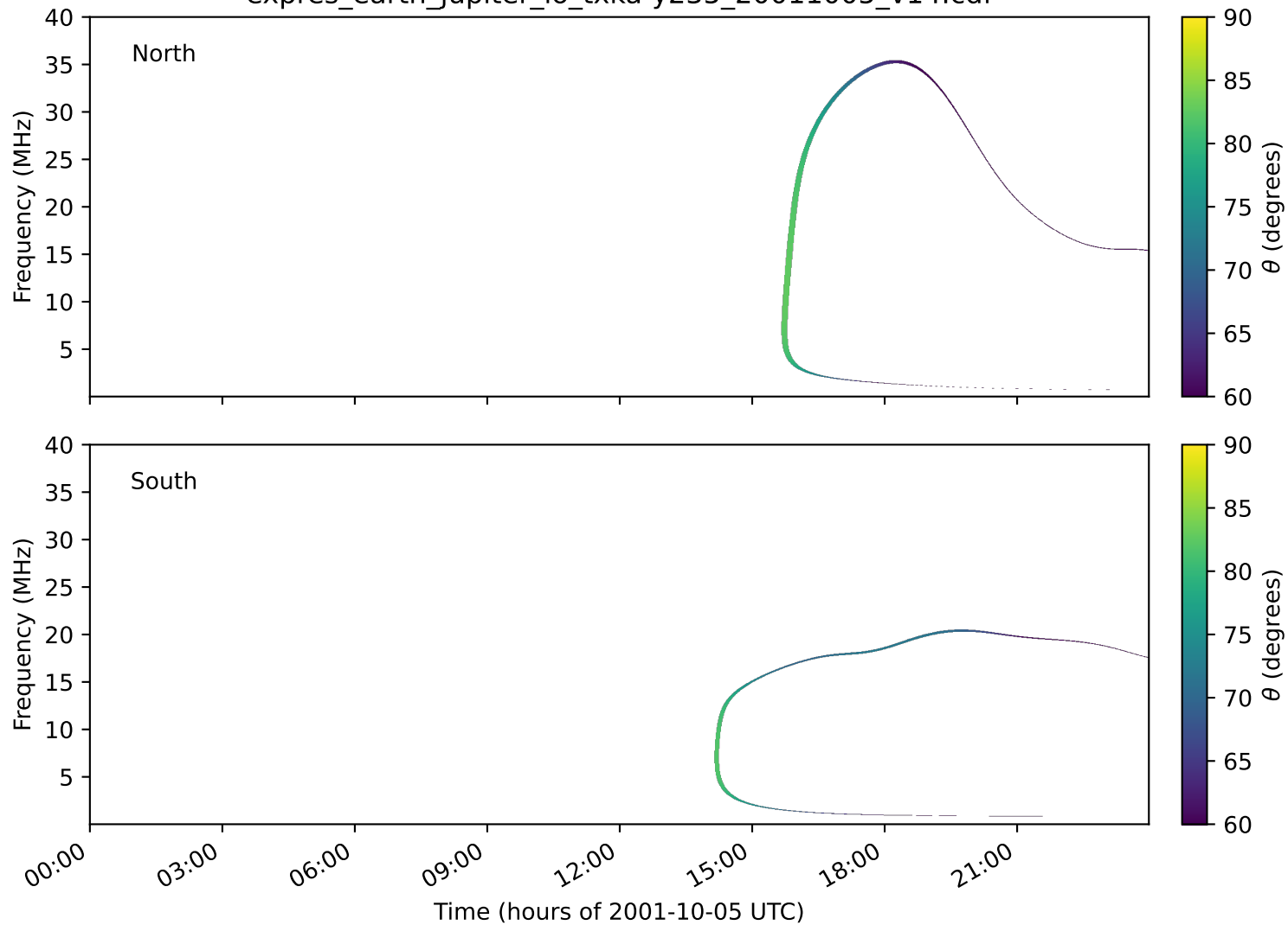
expres_earth_jupiter_io_txka-y235_20011005_v14.cdf
