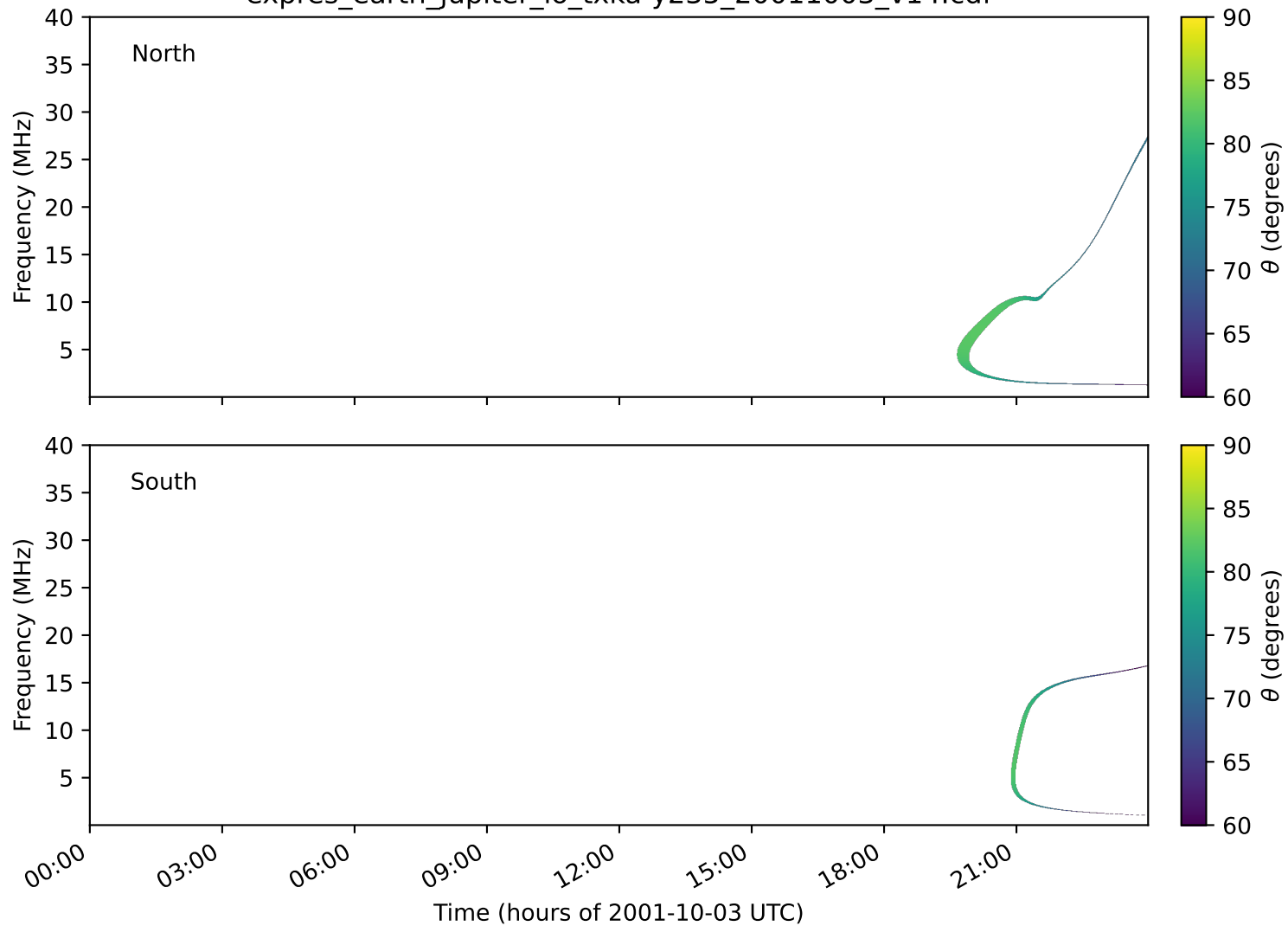
expres_earth_jupiter_io_txka-y235_20011003_v14.cdf
