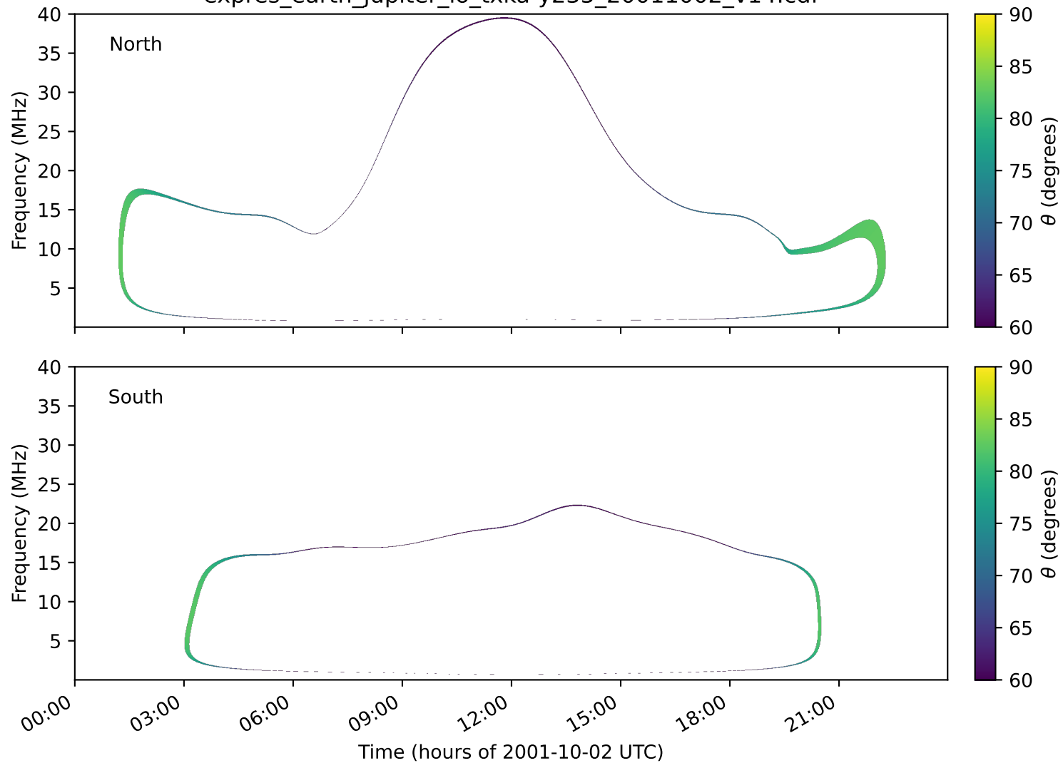
expres_earth_jupiter_io_txka-y235_20011002_v14.cdf
