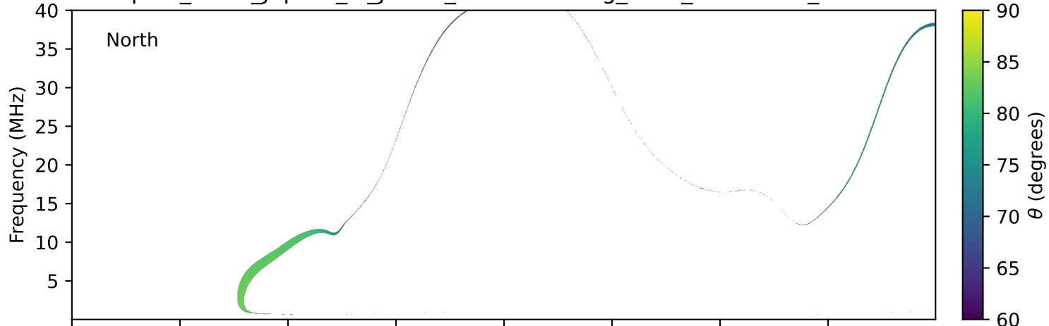
expres_earth_jupiter_io_jrm33_lossc-wid1deg_3kev_20011016_v11.cdf
