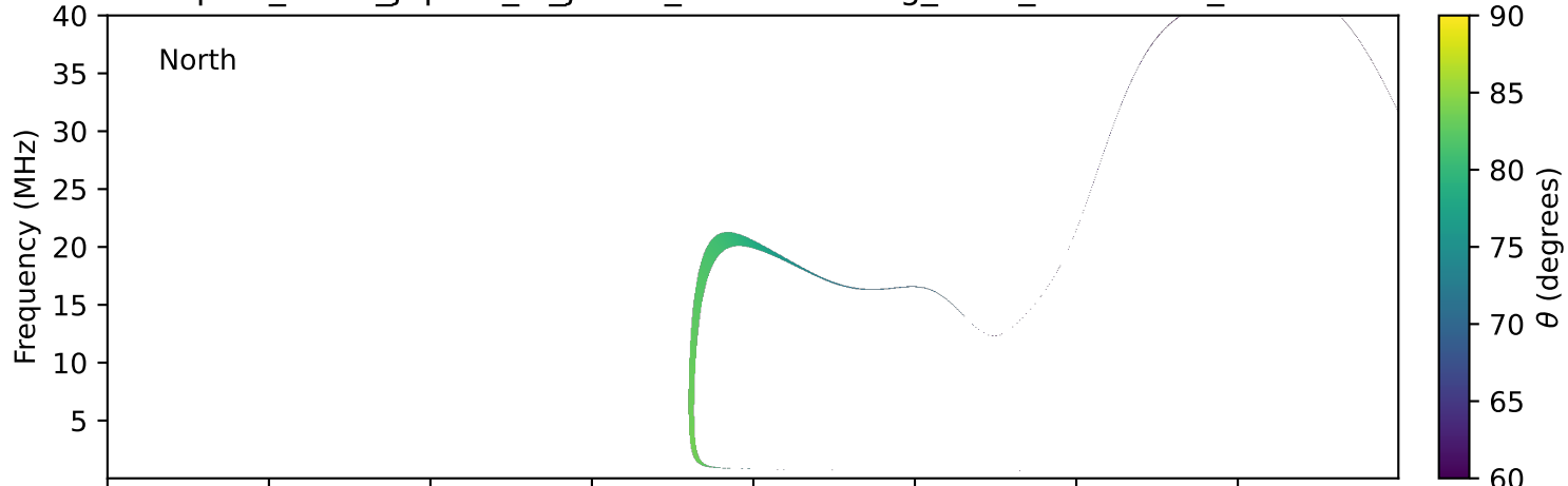
expres_earth_jupiter_io_jrm33_lossc-wid1deg_3kev_20011014_v11.cdf
