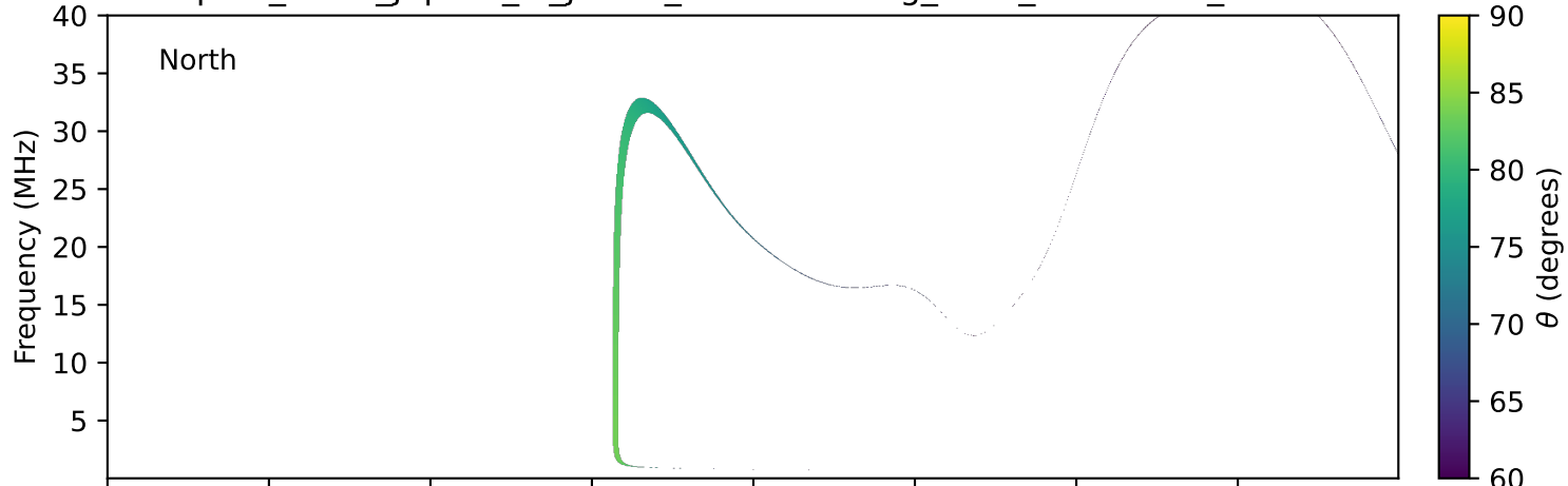
expres_earth_jupiter_io_jrm33_lossc-wid1deg_3kev_20011007_v11.cdf
