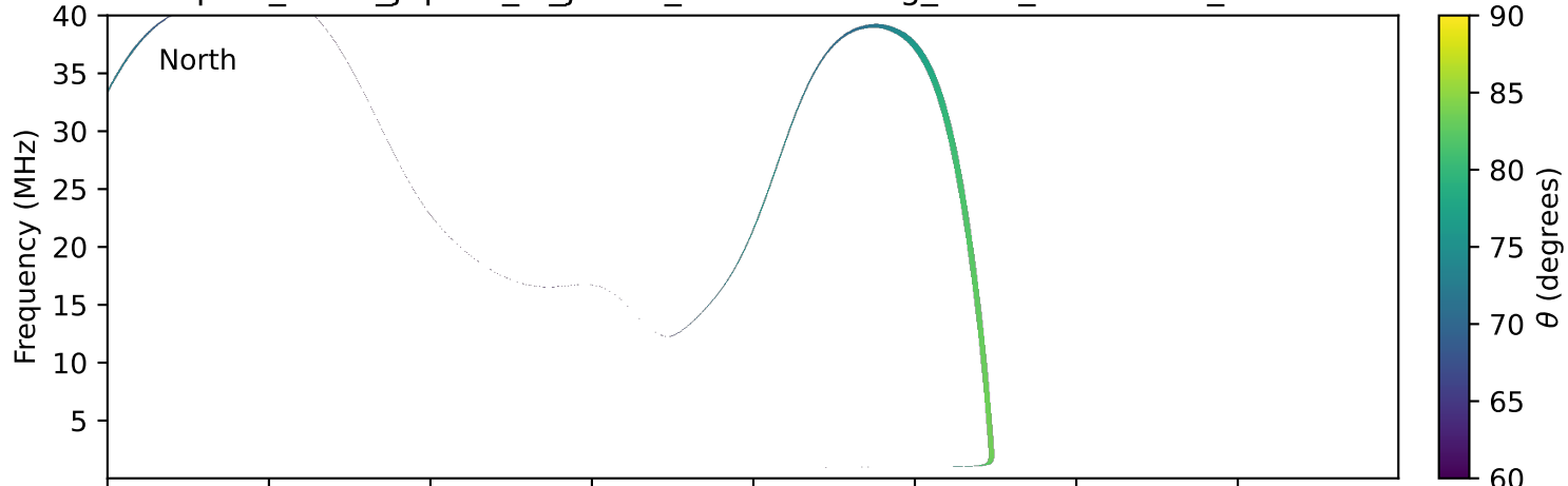
expres_earth_jupiter_io_jrm33_lossc-wid1deg_3kev_20011004_v11.cdf
