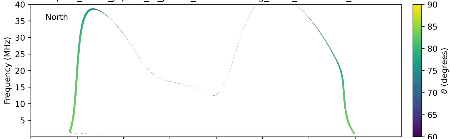
expres_earth_jupiter_io_jrm09_lossc-wid1deg_3kev_20011025_v11.cdf
