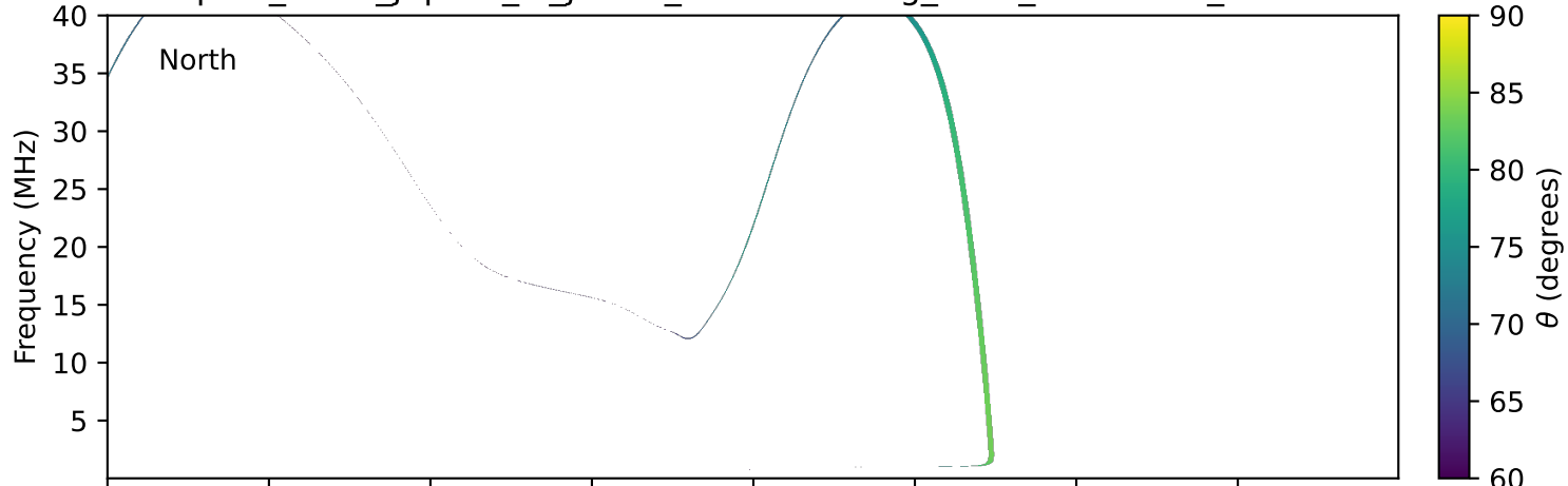
expres_earth_jupiter_io_jrm09_lossc-wid1deg_3kev_20011004_v11.cdf
