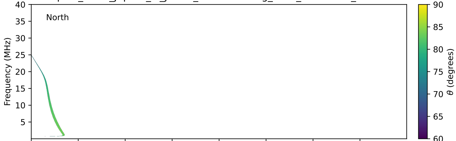
expres_earth_jupiter_io_jrm09_lossc-wid1deg_3kev_20011001_v11.cdf
