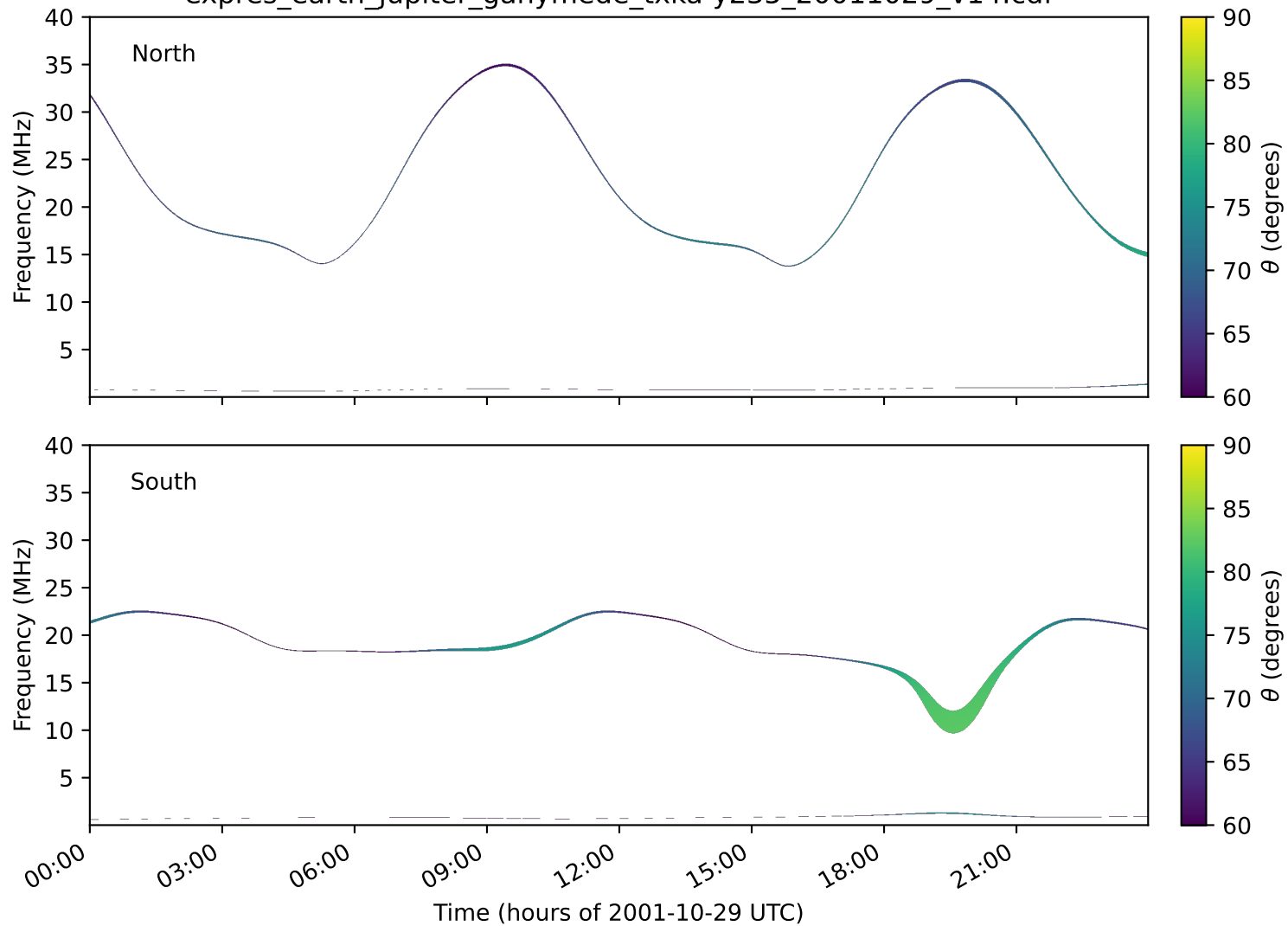
expres_earth_jupiter_ganymede_txka-y235_20011029_v14.cdf
