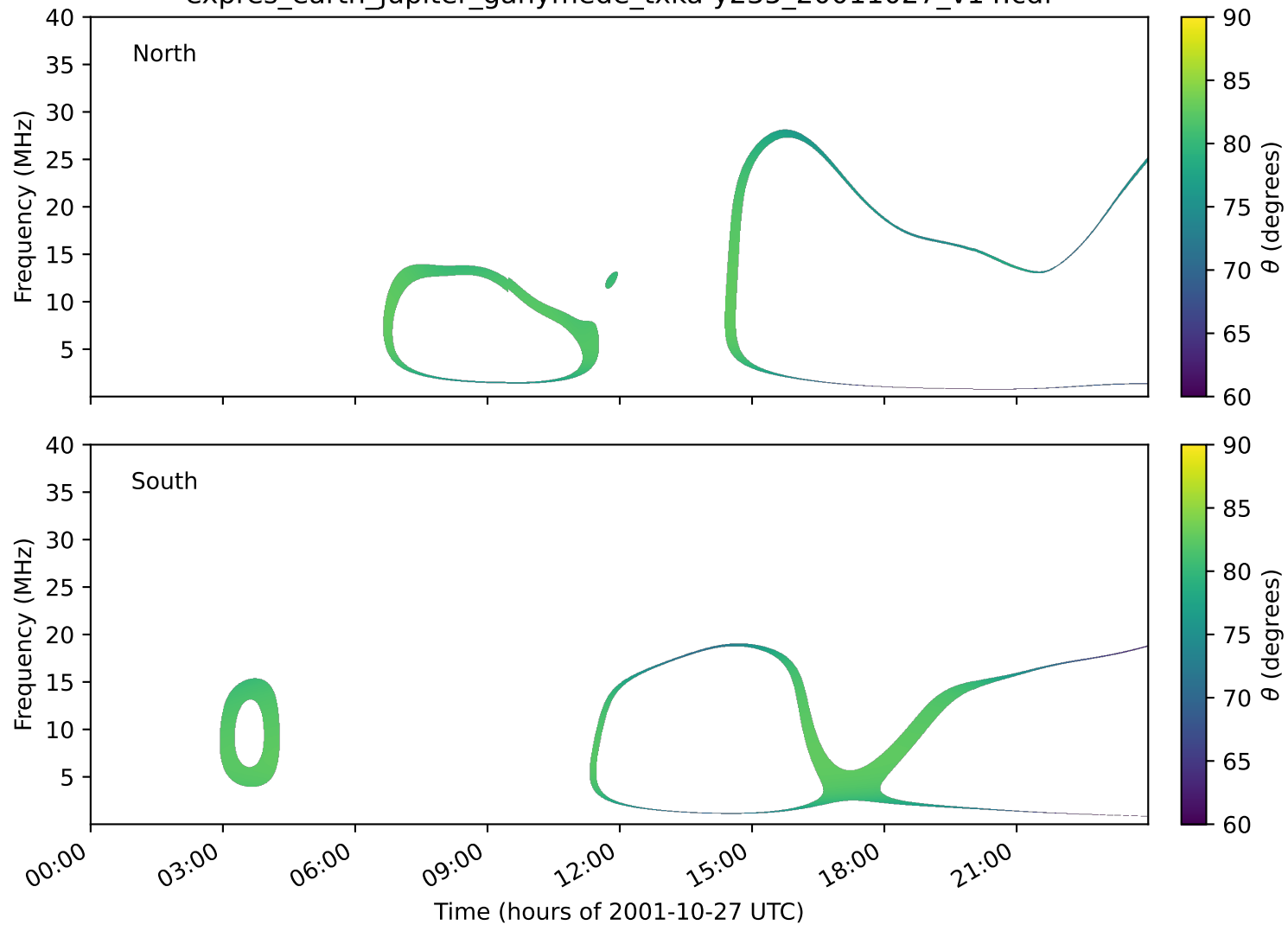
expres_earth_jupiter_ganymede_txka-y235_20011027_v14.cdf
