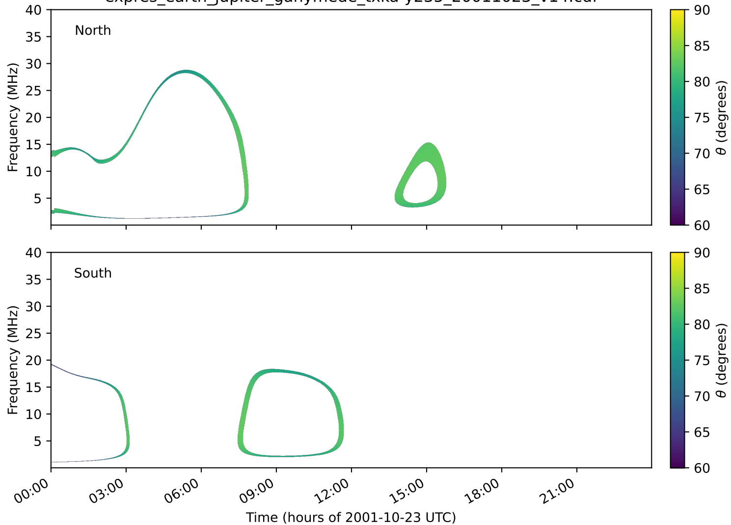
expres_earth_jupiter_ganymede_txka-y235_20011023_v14.cdf
