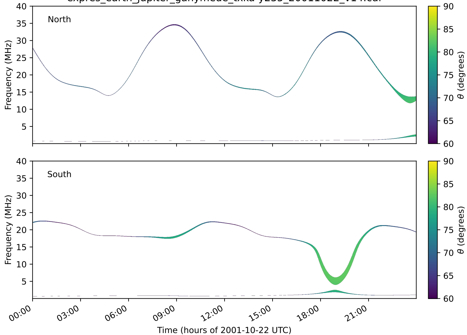
expres_earth_jupiter_ganymede_txka-y235_20011022_v14.cdf
