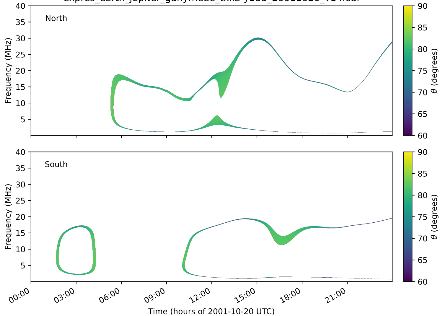
expres_earth_jupiter_ganymede_txka-y235_20011020_v14.cdf
