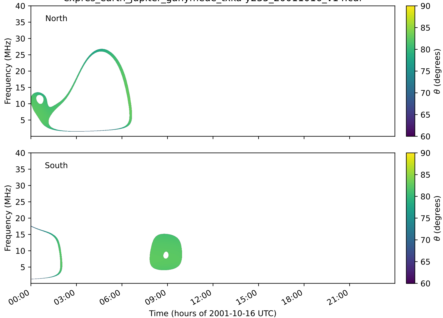
expres_earth_jupiter_ganymede_txka-y235_20011016_v14.cdf
