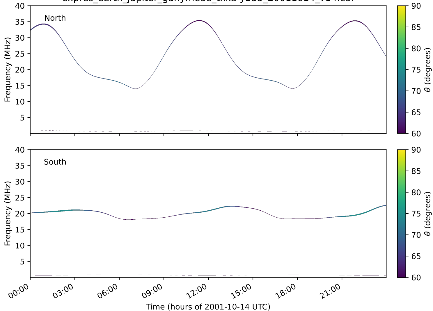
expres_earth_jupiter_ganymede_txka-y235_20011014_v14.cdf
